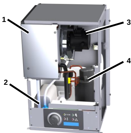
Fig. 3: Vista interior
