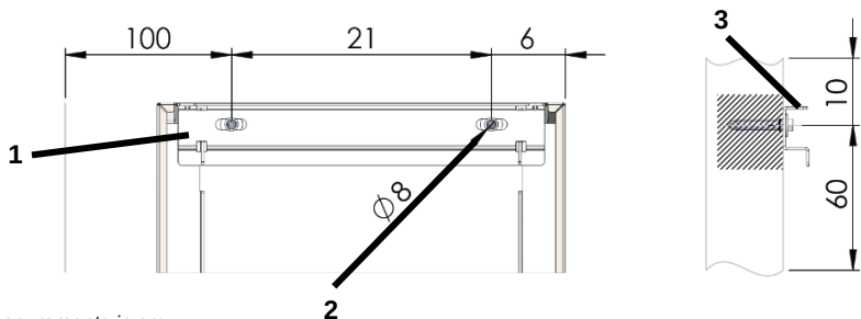
Fig 5: Overview of wall attachment
